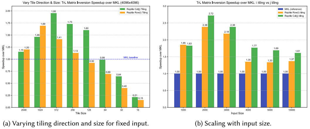
Fig. 21. Triangular Matrix Inversion Speedup over MKL. (a) explores different tile sizes and tiling directions for a 4096x4096 matrix; (b) shows speedups with different matrix sizes.
