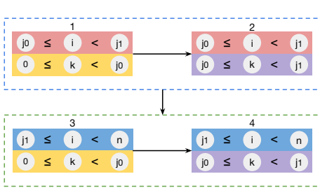
Fig. 10. The Cholesky recurrence system is intersected with the given tiling bounds. The result is a simplified recurrence, which computes an SYRK, i.e. the part of the original recurrences corresponding to these bounds.
